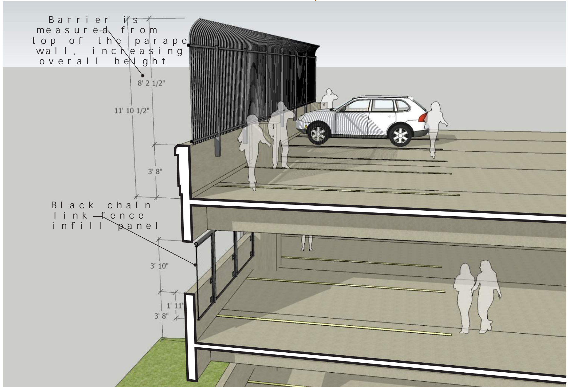
OPTI ON 3 Barrier measured from top of parapet sill
