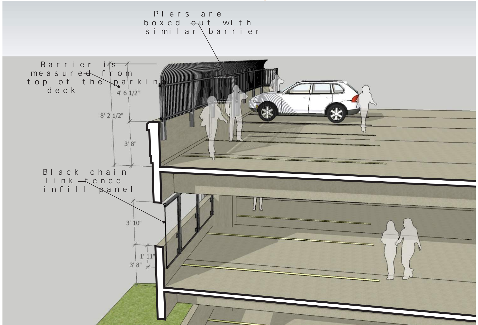
OPTI 01 Barrier measured from the top of the deck, piers with similar barrier.
