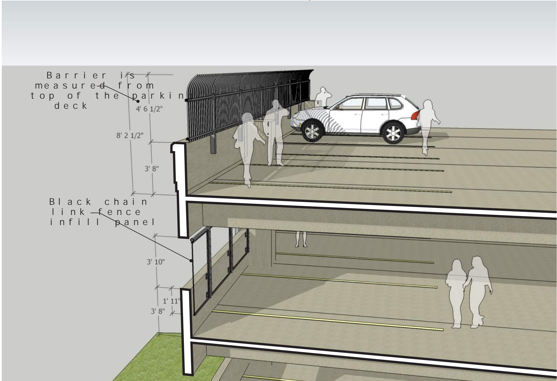
OPT I O N 1 6 Barrier measured from the top of the deck, running
